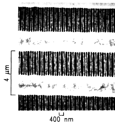
FIG. 3. Scanning electron microscope micrograph of a portion of the grating that was damaged during mounting.
