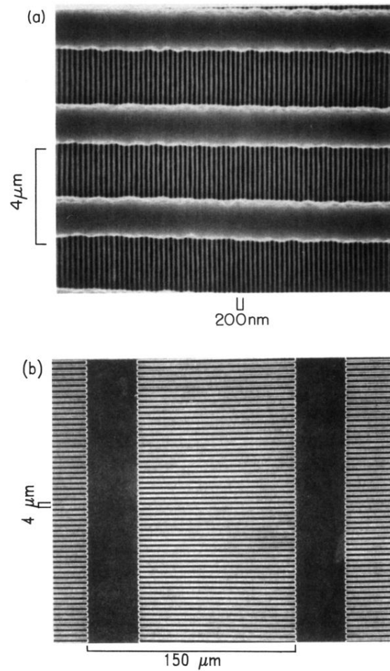
FIG. 1. Scanning-electron-microscope micrographs of the completed grating at two different scales. (a) 0.2- \mu\text{m} period grating overlaid with the 4- \mu\text{m} period grating. (b) 150 \times 4- \mu\text{m}^2 support grid on a larger scale.
