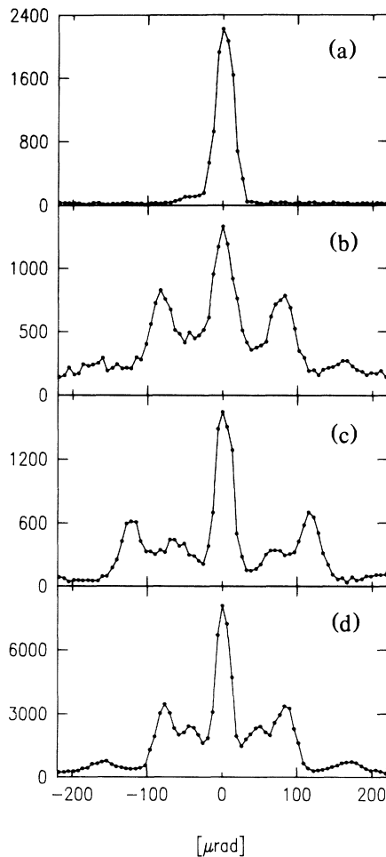
FIG. 2. Experimental profile of the Na beam. The y axes are the number of detected atoms; the counting time at each point is \sim 1 \text{ sec} . The line through the points is only for visual effect. As explained in the text, (a) is the undiffracted beam, and (b)–(d) show the beam diffracted by transmission through the grating. In (c) the carrier gas is Xe, in the other cases it is Ar.
