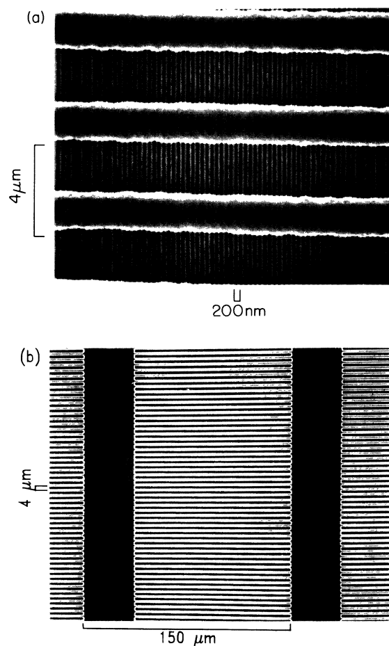
FIG. 1. Scanning-electron-microscope micrographs of the completed grating at two different scales. (a) 0.2- \mu\text{m} period grating overlaid with the 4- \mu\text{m} period grating. (b) 150 \times 4- \mu\text{m}^2 support grid on a larger scale.
