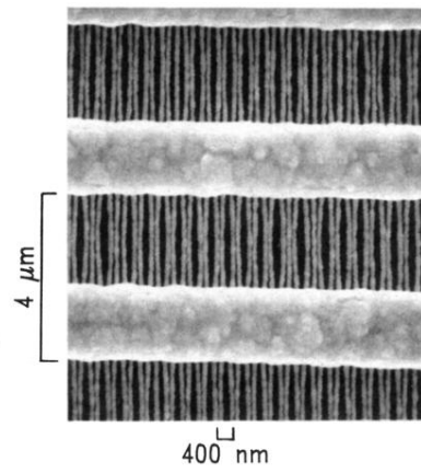
FIG. 3. Scanning electron microscope micrograph of a portion of the grating that was damaged during mounting.
