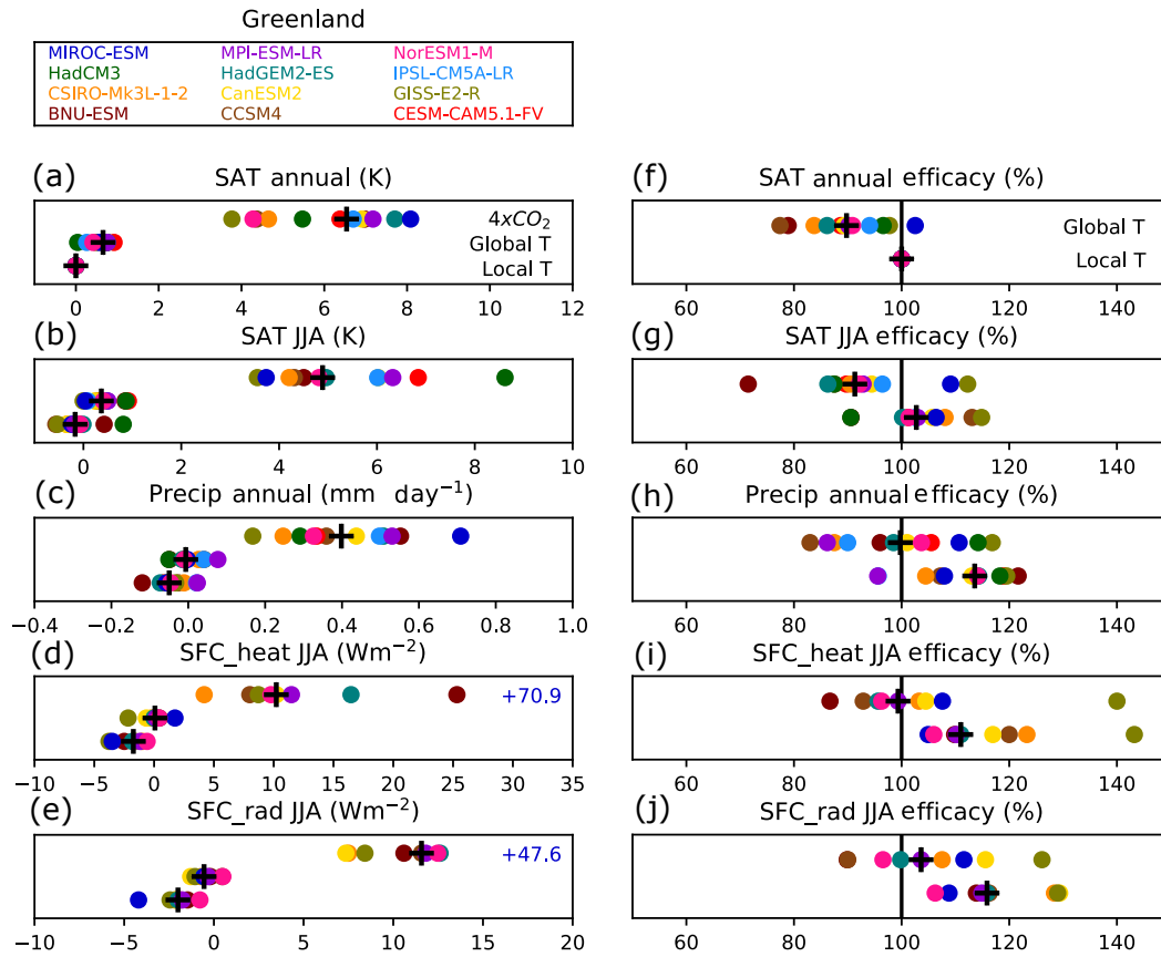
Figure 1. Regional-mean anomalies (a–e) and efficacies (f–j) of G1* and G1-Greenland at offsetting 4 × CO 2 – control regional-mean anomalies for Greenland for each model within the GeoMIP G1 ensemble. In (a–e), the upper points show the 4 × CO 2 – control anomaly, the middle row of points show the G1* results, which restore global mean temperature, and the lower points show the results for G1-Greenland, which restores local temperature. The ensemble median is shown with a plus symbol. The results from some outlier points have been displayed as text in the color of the corresponding model. SFC heat is the net heat flux into the surface, i.e., net SW + net LW – sensible heat – latent heat, and SFC rad is the net radiative flux into the surface, i.e., net SW + net LW. Efficacy is defined in the text. Where data were unavailable these models have not been plotted for those variables.
