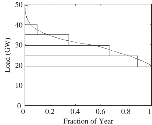
Fig. 1. Year 2000 load duration curve for the MAAC NERC region (the PJM system) and its discretized approximation. The curve represents the fraction of the year that hourly electricity demand in 2000 exceeded a given level (PJM, 2001). Explicit seasonal variation in peak and baseload levels is thus ignored. Demand growth in subsequent periods follows EIA projections (EIA, 2001a), although the shape of the load-duration curve remains constant.
