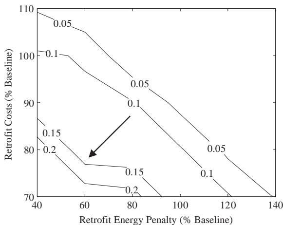
Fig. 7. Fraction of electricity produced in period 6 (2026–2030) by retrofit coal plants as a function of retrofit costs and energy penalty under a 150$/tC emissions price. Costs include capital plus fixed and variable O&M, and both sets of model parameters are shown as a percentage of their baseline specifications (see Table 2). Note that lower emission prices decrease coal plant conversions (as with CCS in general), while higher prices do not increase the share of retrofit generated power. The arrow indicates the direction of increasing retrofit penetration.
