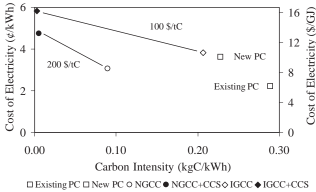
Fig. 4. Total cost of electricity versus carbon emissions per unit of energy generated. Total cost is defined as the sum of marginal and fixed operating expenses and a capital recovery charge. (Existing PC is assumed to be fully amortized and therefore does not include the latter.) The slope of the line connecting a given plant (defined by generating technology and fuel choice) with its CO 2 -capture equivalent is the emissions price threshold above which the latter is preferred. Conventional coal plants, for instance, would be less expensive to build and operate until the value of CO 2 reaches 100$/tC, beyond which carbon capture dominates. Likewise, carbon capture for new gas facilities is not economical until the carbon price approaches 200$/tC. A load factor of 90 percent is assumed for all technologies; fuel prices and technology specifications are that of the unconstrained carbon emission base model (see Tables 1 and 2). (“Existing PC”—average existing amortized pulverized coal plant; “New PC”—new conventional pulverized coal plant; “IGCC”—integrated gasified (coal) combined cycle; “NGCC”—combined cycle natural gas turbine; “+ CCS”—with carbon capture and sequestration.)
