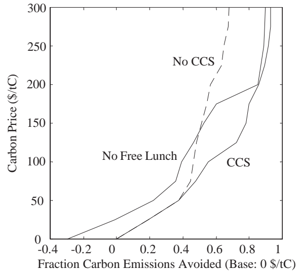
Fig. 5. Carbon mitigation cost curves when CCS technologies are available (“CCS”) and when they are not (“No CCS”), as well as when the free lunch CO 2 reduction of fuel switching is removed (“No Free Lunch”). The mitigation cost curves represent a series of model runs, with carbon prices increasing from 0 to 300$/tC in 10$/tC increments. The discrete points on the curve reflect the reduction in 2001–2040 emissions under a given carbon price and 0$/tC, expressed as a fraction of the latter (2.07 GtC). This approach to generating a mitigation supply curve is equivalent to imposing a constraint on CO 2 emissions and plotting the increase in undiscounted total costs as a function of the corresponding emissions reduction. Note that the zero-carbon price emissions level of the baseline run (2.07 GtC) provides the basis used to calculate the fraction of CO 2 avoided for the “No Free Lunch” scenario.
